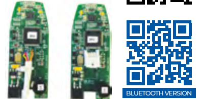
MA1 13.56 MHz High security mullion module Built-in antenna
